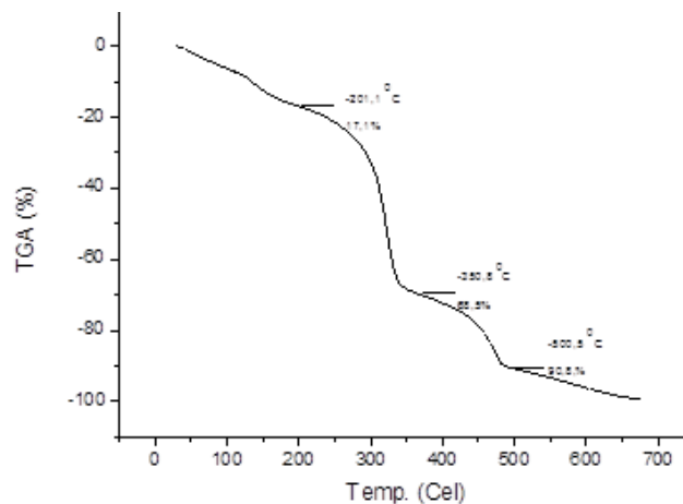
Figure 14 The TGA Spectrum of TPSS/LLDPE Compatibilized blends
